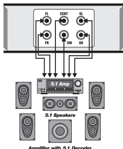
Amplifier with 5.1 Decoder
