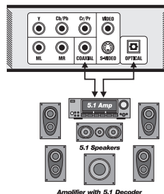
Amplifier with 5.1 Decoder
